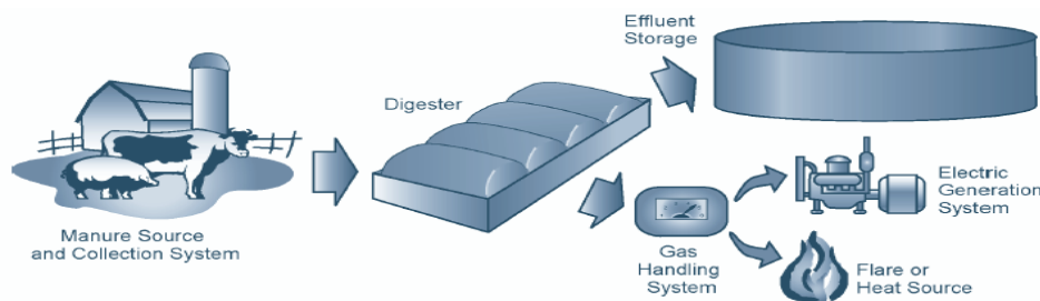
Figure VII-7 Biogas Recovery Systems
